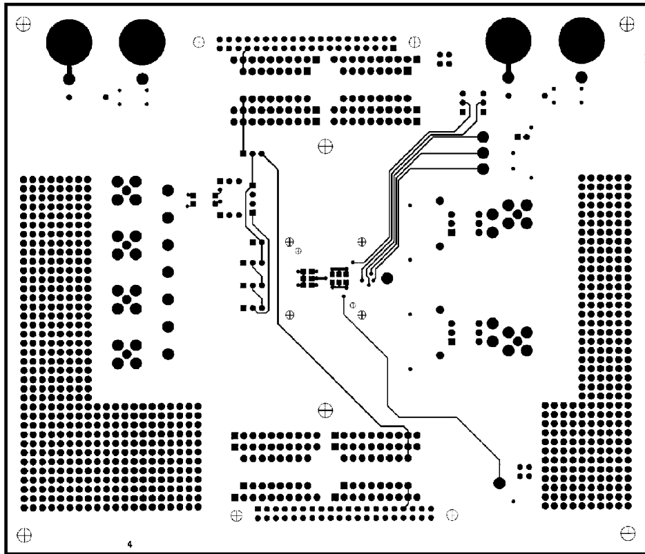
Figure 94. Layer 4, Bottom Side
