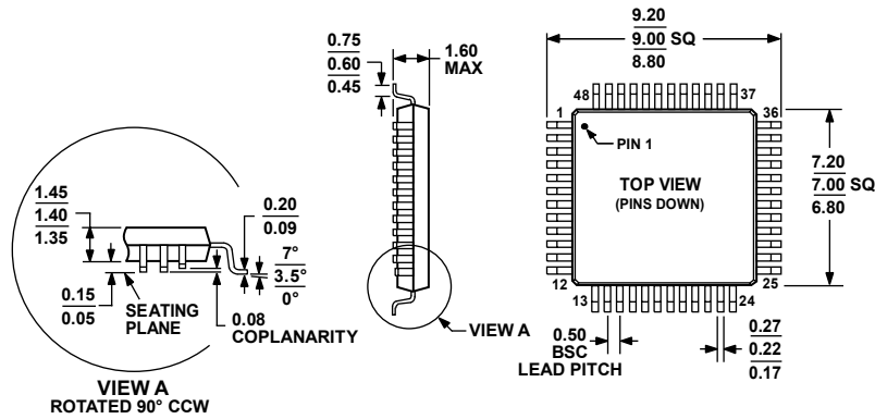
Figure 95. 48-Lead Low Profile Quad Flat Package [LQFP] (ST-48)
