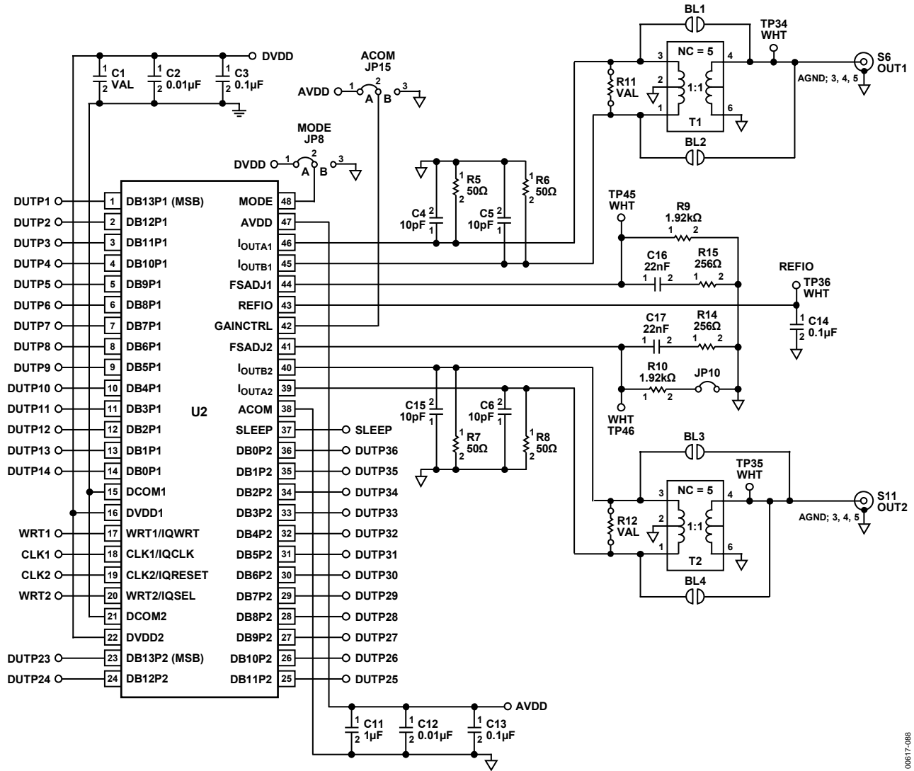
Figure 88. AD9767 and Output Signal Conditioning
