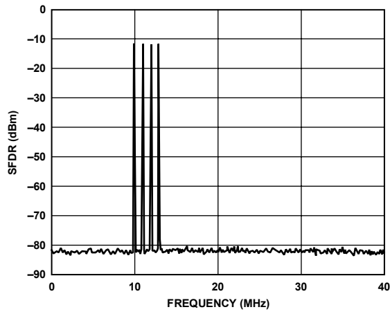
Figure 22. Four-Tone SFDR @ f CLK = 125 MSPS
