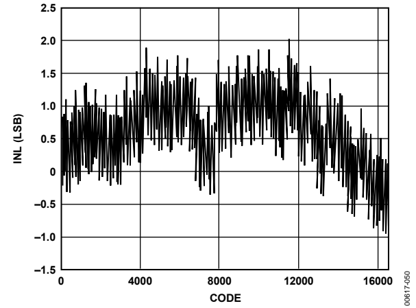
Figure 50. Typical INL
