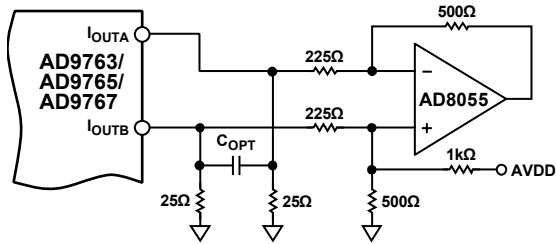
Figure 74. Single-Supply DC Differential-Coupled Circuit
