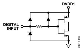
Figure 67. Equivalent Digital Input
