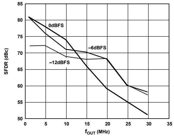
Figure 26. SFDR vs. f_{OUT} @ 65 MSPS
