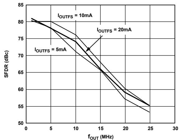
Figure 28. SFDR vs. f_{OUT} and I_{OUTFS} @ 65 MSPS and 0 dBFS
