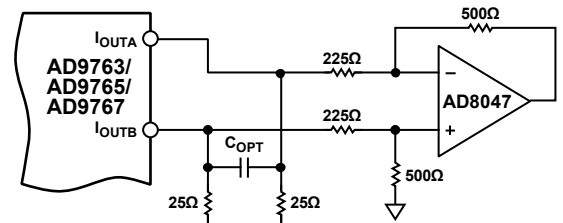
Figure 73. DC Differential Coupling Using an Op Amp
