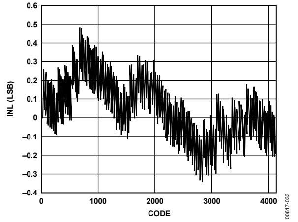
Figure 33. Typical INL
