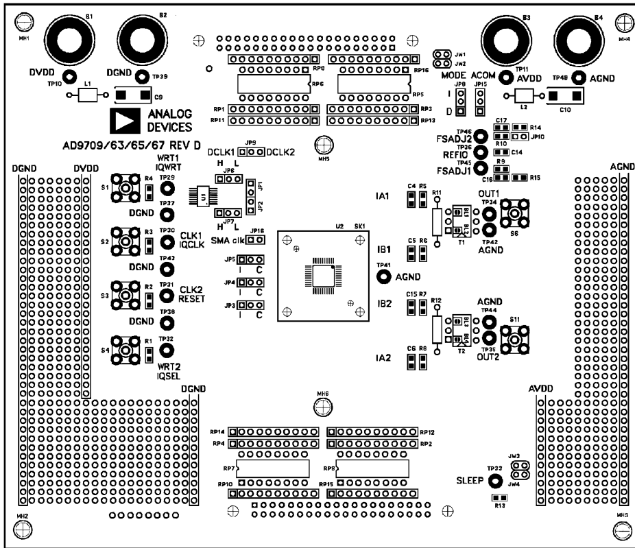
Figure 89. Assembly, Top Side
