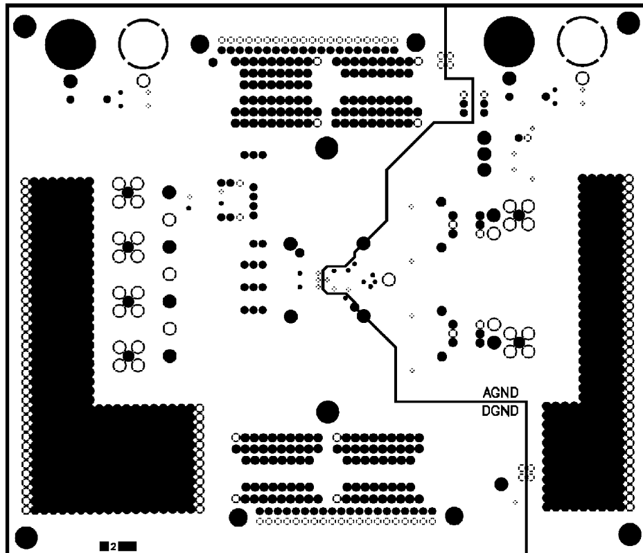
Figure 92. Layer 2, Ground Plane
