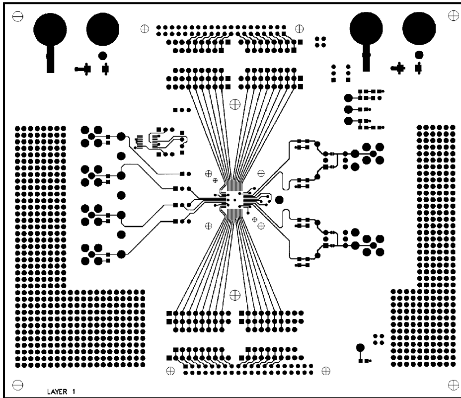
Figure 91. Layer 1, Top Side
