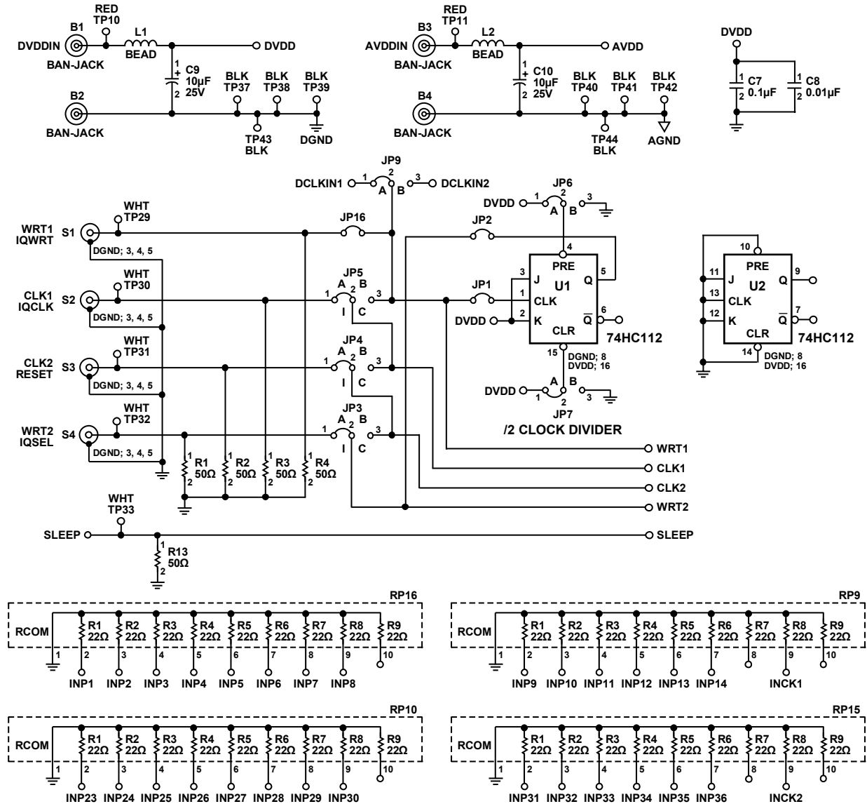
Figure 86. Power Decoupling and Clocks on AD9763/AD9765/AD9767 Evaluation Board
