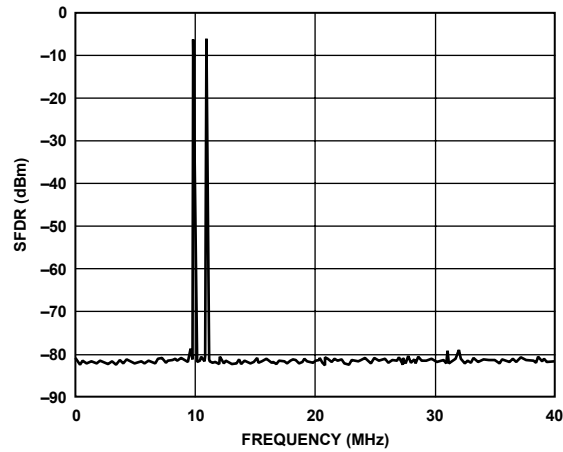
Figure 21. Dual-Tone SFDR @ f CLK = 125 MSPS
