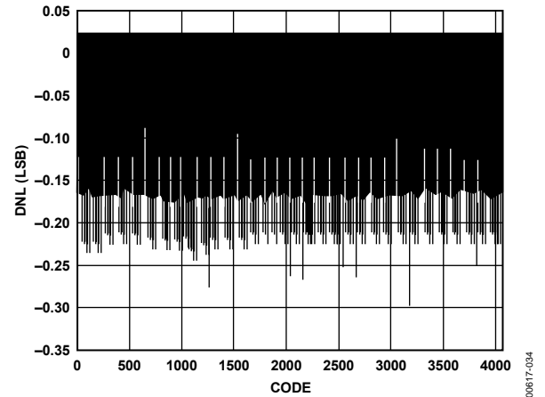
Figure 34. Typical DNL
