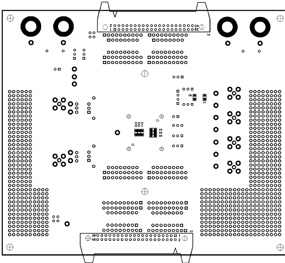
Figure 90. Assembly, Bottom Side
