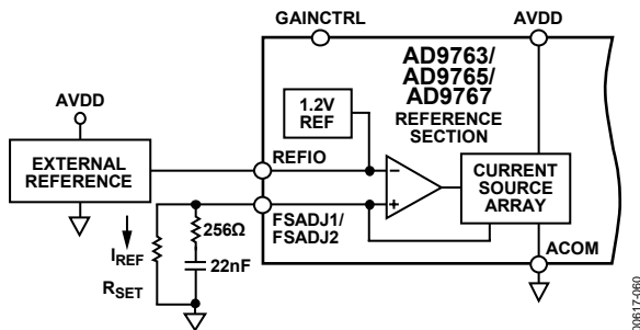
Figure 60. External Reference Configuration Gain Control Mode
