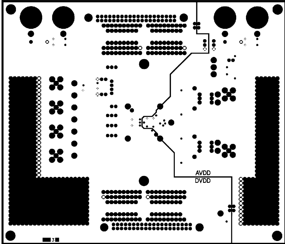
Figure 93. Layer 3, Power Plane
