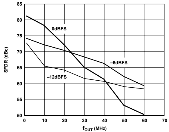
Figure 27. SFDR vs. f_{OUT} @ 125 MSPS
