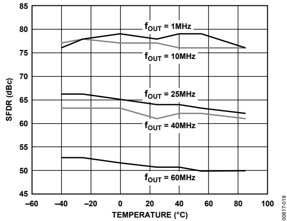
Figure 18. SFDR vs. Temperature @ f CLK = 125 MSPS, 0 dBFS
